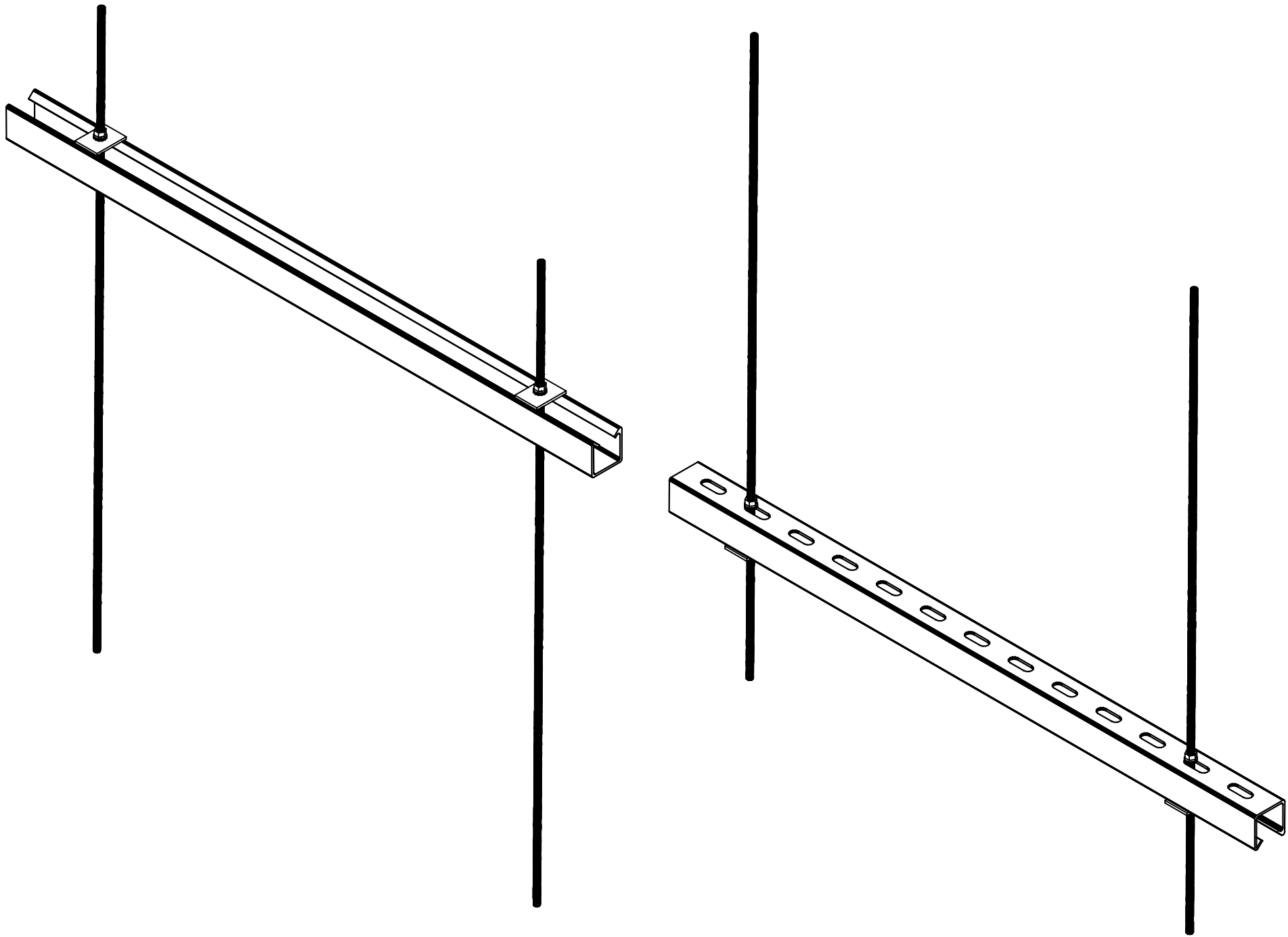
9) C CHANNEL SUPPORT / ROD BOLT
