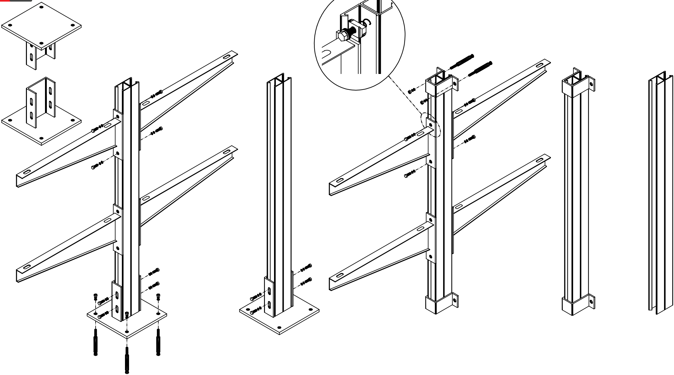
8)C CHANNEL SUPPORT DOUBLE/HOLDER/POST BASE
