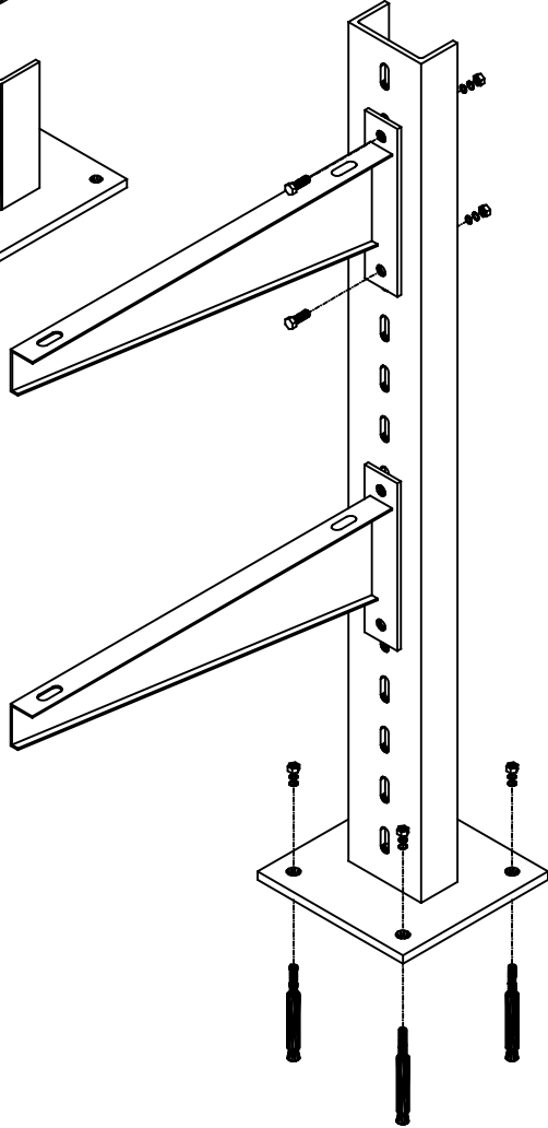
1)U SUPPORT/BASE PLATE/POST BASE
