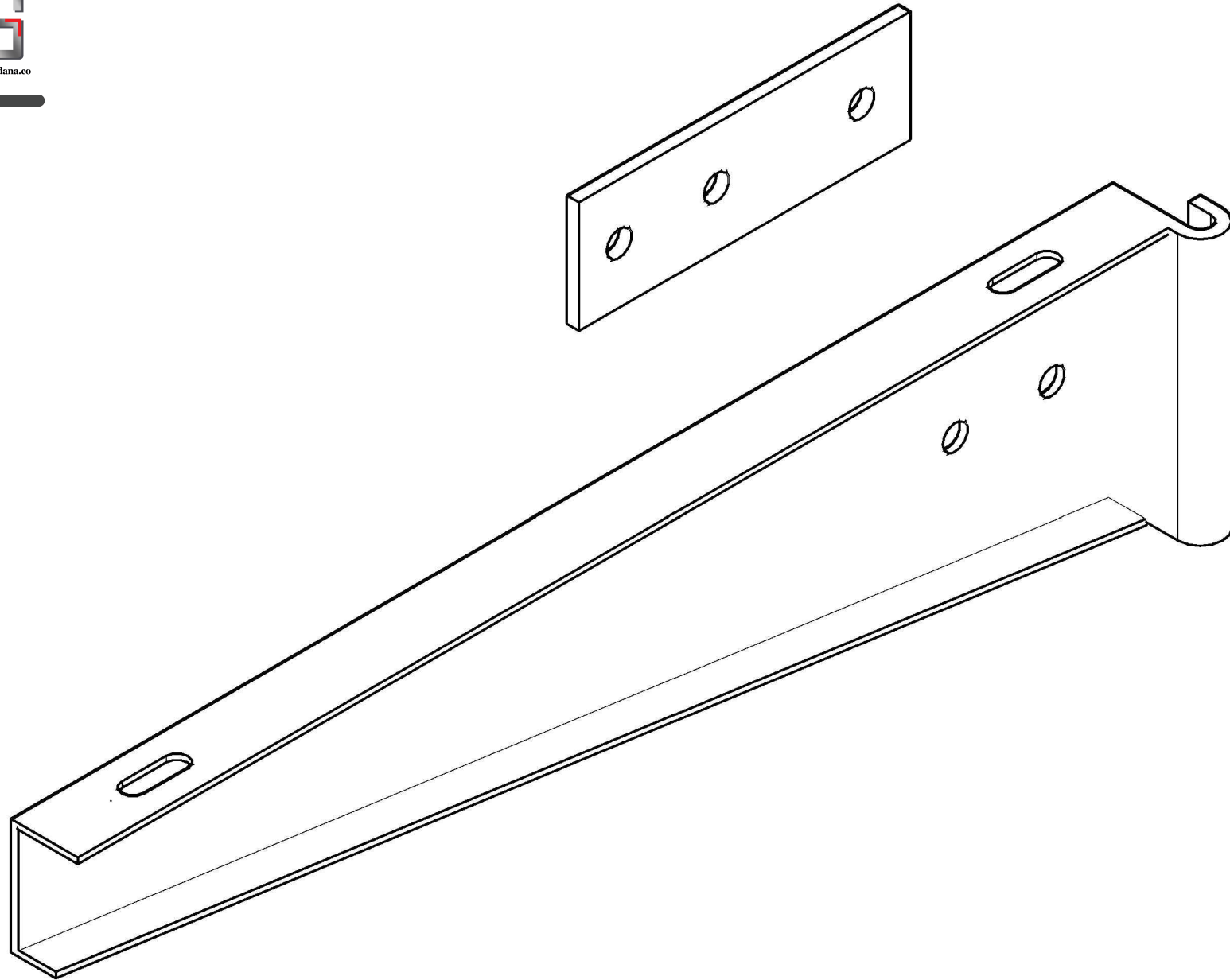
2)GRIPPING BRACKET
